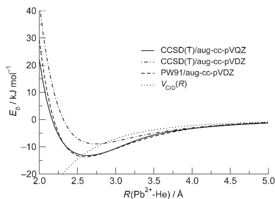
Figure 1. Potential energy curves for \text{PbHe}_N^{2+} using various theoretical methods. The CID curve is also shown. Binding energies E_b and bond lengths R_b : CCSD(T)/aug-cc-pVQZ 13.22 \text{kJ mol}^{-1} and 2.629 Å; CCSD(T)/aug-cc-pVDZ 8.97 \text{kJ mol}^{-1} and 2.738 Å; PW91/aug-cc-pVDZ 13.70 \text{kJ mol}^{-1} and 2.595 Å.
