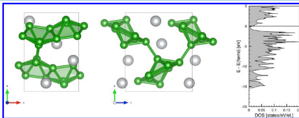
Figure 7. (Left) Two views of the P2_12_12_1 ground state structure of \text{BeB}_4 . Capped B pentagons are shaded. (Right) Electronic DOS, featuring a severe depletion of states at the Fermi energy.
