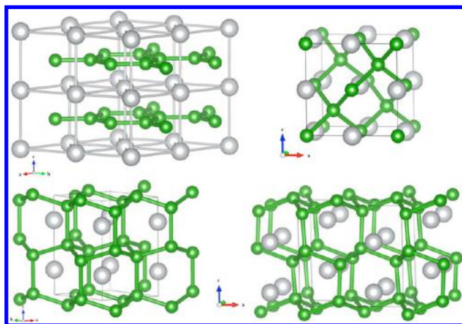
Figure 1. BeB 2 crystal structures. From top left to bottom right: AlB 2 , F 43 m , CaIn 2 , and Pnma structures (see text for details). All are optimized structures at P = 1 atm. Note the buckled boron layers in the two structures in the bottom panel. Small green (large gray) spheres denote boron (beryllium) atoms.
