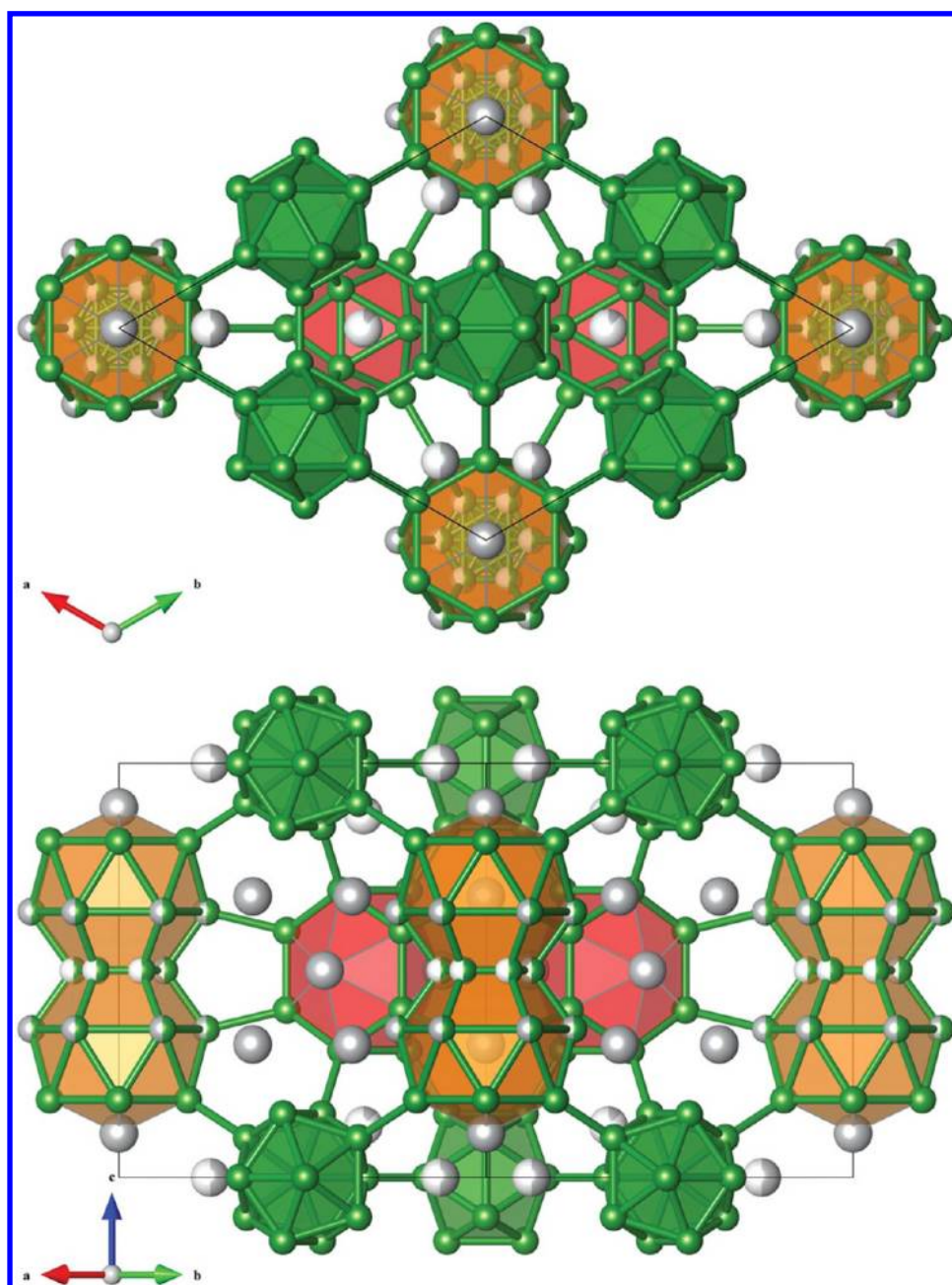
Figure 8. Experimental crystal structure of " \text{BeB}_{2.75} " at T = 120 \text{ K} , 4 seen along the c axis (top) and within the a – b plane (bottom). Green (gray) spheres denote boron (beryllium) atoms, and partially filled spheres indicate partially occupied lattice sites. Green polyhedra indicate \text{B}_{12} icosahedra, red polyhedra the \text{Be}_3\text{B}_{12} subunits, and orange polyhedra the \text{Be}_8\text{B}_{21} subunit with most of the partial occupancies (see text).
