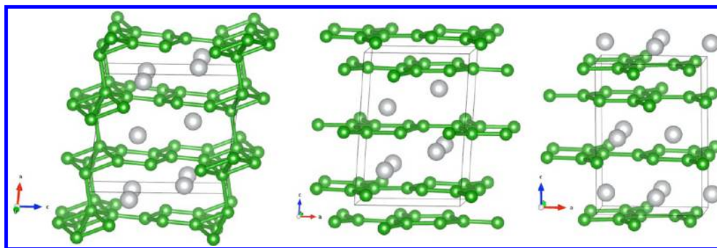
Figure 4. Predicted \text{BeB}_3 crystal structures: (left) C2/m phase; (middle) P2_1/m phase; (right) Cm phase. All shown to the same scale and optimized at P = 1 atm.
