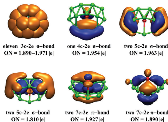
Fig. 5 AdNDP bonding pattern of the neutral ZrB_{12} cluster, ON stands for occupation number.
