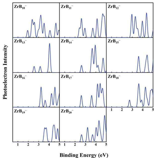
Fig. 2 The simulated photoelectron spectra of anionic \text{ZrB}_n^- ( n = 10\text{--}20 ) clusters.
