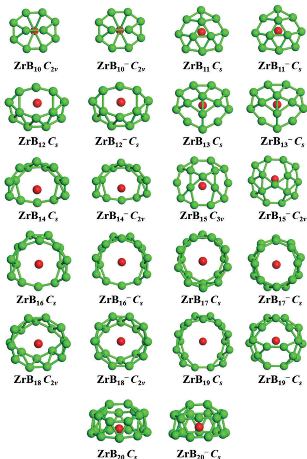
Fig. 1 Lowest-energy structures of ZrB_n^Q ( n = 10-20 , Q = 0, -1 ) clusters along with their point group symmetries.
