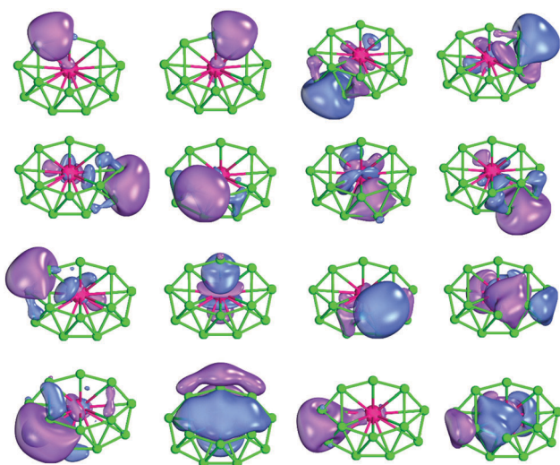
Fig. 4 The intrinsic bond orbitals of the neutral ZrB_{12} cluster visualized by IboView. 61 The iso-surfaces enclose 80% of the orbitals' electron density.
