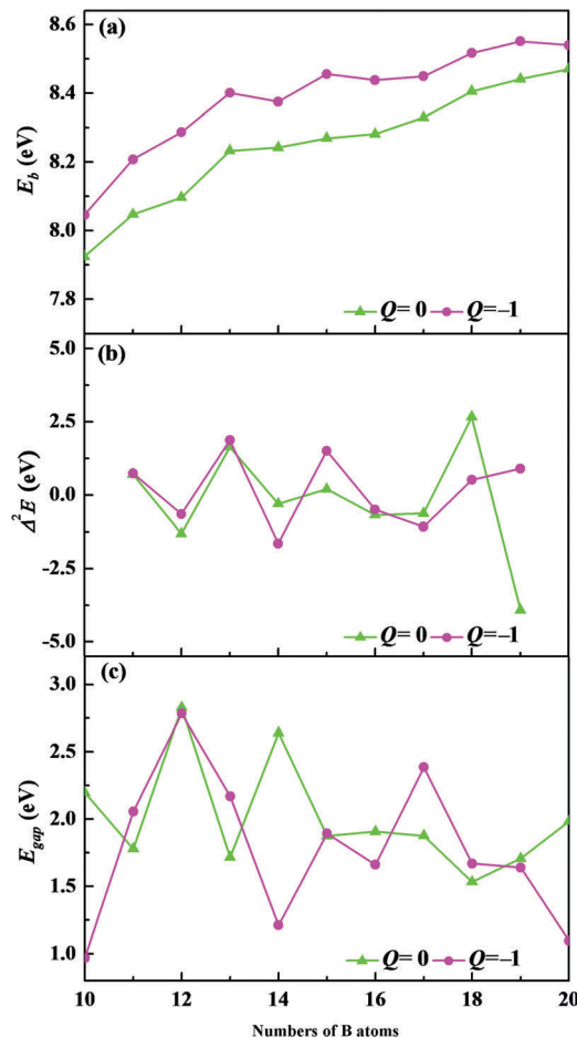
Fig. 3 The (a) binding energy per atom ( E_b ), (b) second energy difference ( \Delta^2E ) and the (c) HOMO–LUMO gap ( E_{\text{gap}} ) for the lowest-energy neutral and anionic \text{ZrB}_n^Q ( n = 10\text{--}20 , Q = 0, -1 ) clusters.
