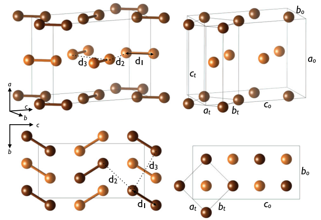
FIG. 1 (color online). Left: Molecular Cmca phase of the halogens, with shortest atomic distances indicated. Right: the unit cell of the atomic I4/mmm phase (lattice a_t, b_t, c_t ) in relation to the Cmca unit cell (lattice a_o, b_o, c_o ). Side-on and top views are given, respectively. Different shades denote atoms in different layers.
