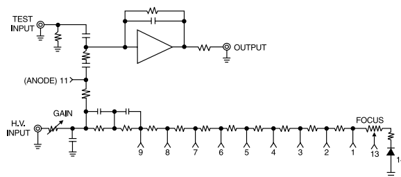
Model 2007P Functional Schematic
